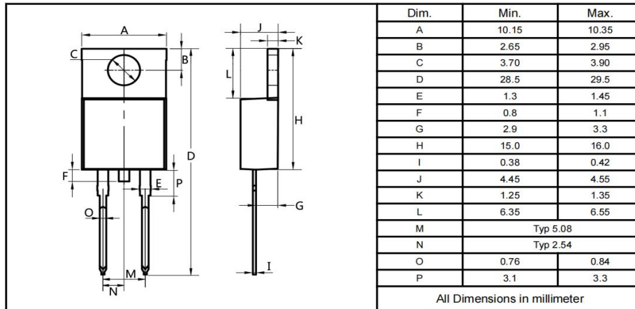
TO-220FAC
